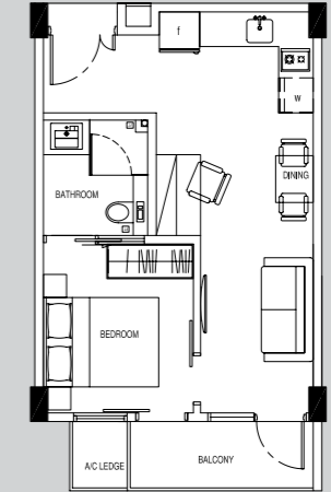
TYPE B (40 sqm)/(431 sq ft)
