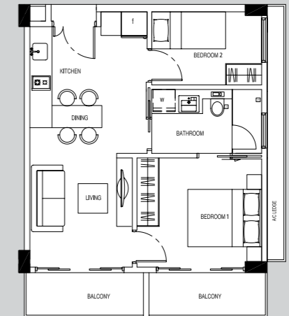
TYPE D (59 sqm)/(635 sq ft)
